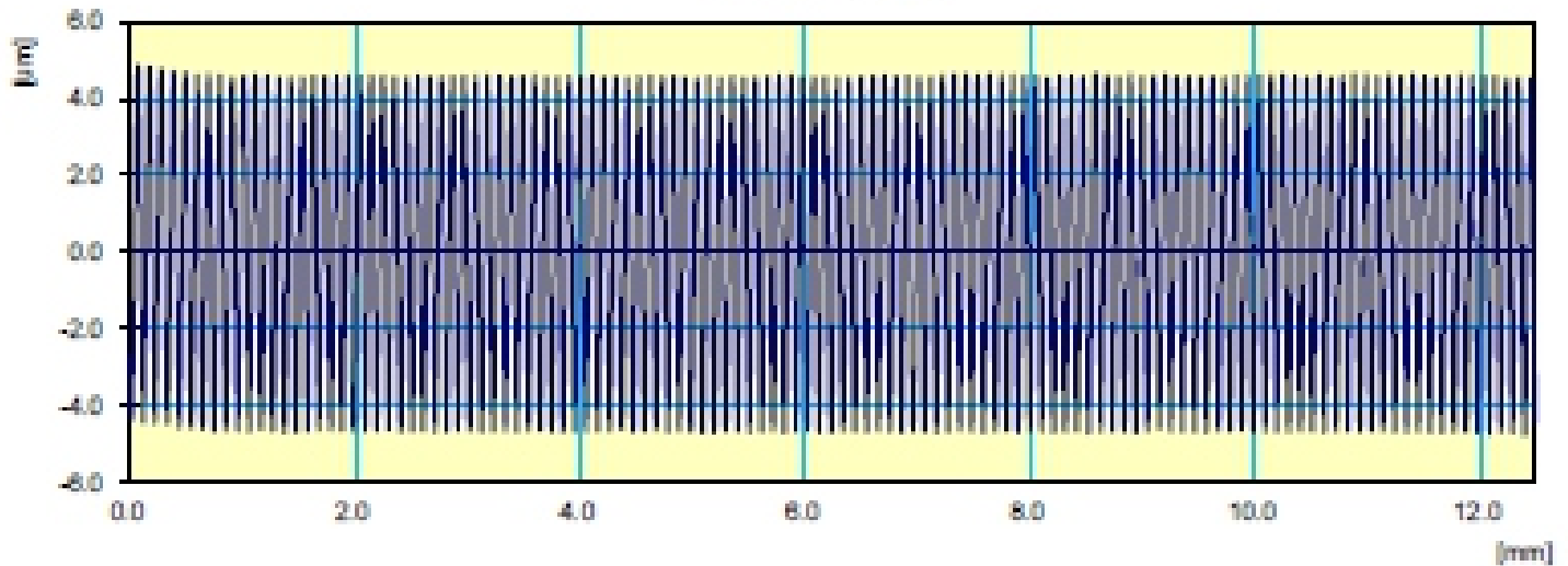
Evaluation Profile
